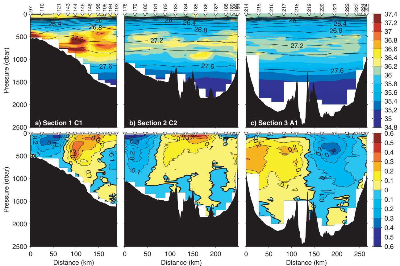
Figure 2. Vertical sections of (upper panels) salinity (color shading) and density ( \sigma_\theta ; contours) and (lower panels) cross-section component of LADCP velocity (in \text{m s}^{-1} ) for the three eddies as shown in Figure 1. North end of each section is on left. Station locations and numbers are indicated along top axes.
