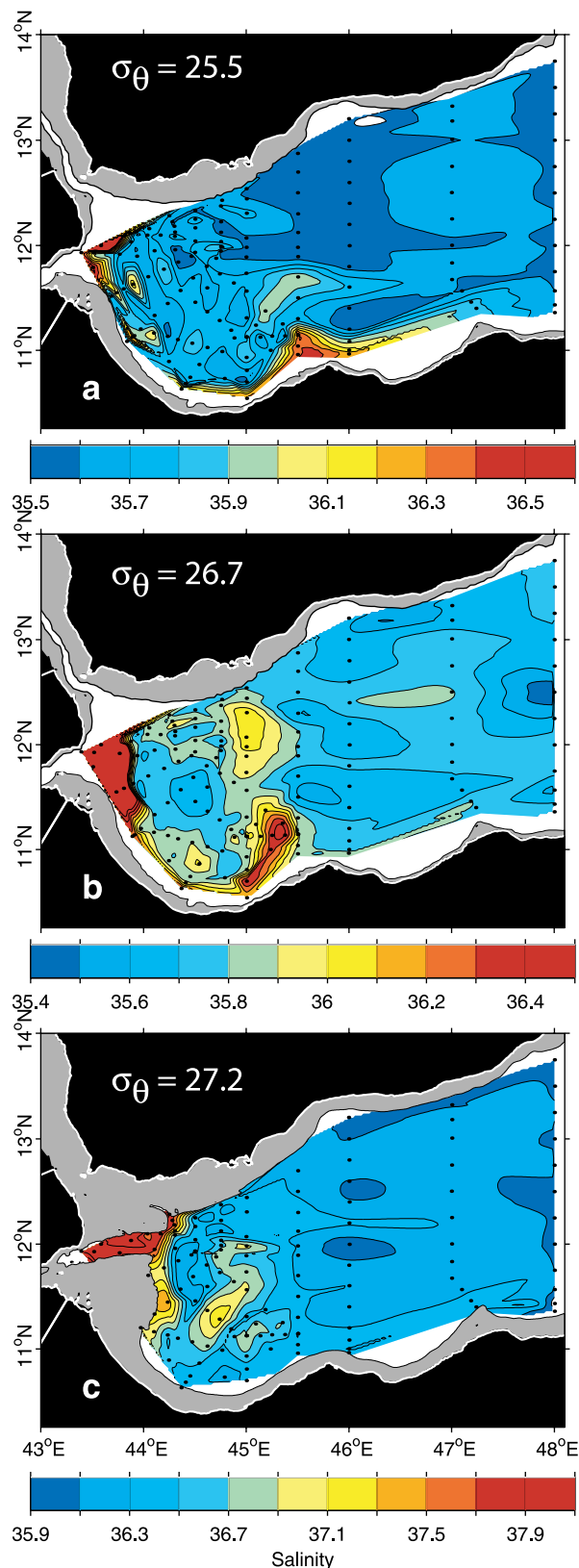
Figure 3. Salinity distribution in the western Gulf of Aden on three density surfaces, \sigma_\theta = 25.5 , 26.7 and 27.2 , at nominal depths of 100, 300 and 600 m. Note that the salinity range and contour interval in (c) are twice that in (a) and (b).
